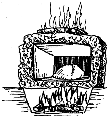
A large tin, banked with clay, makes an effective rough oven.
