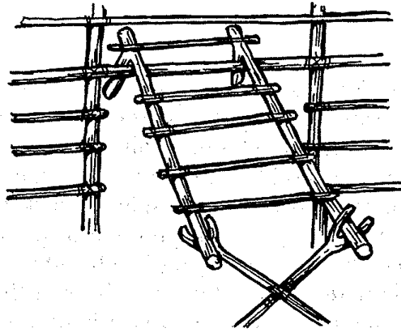
The method of making window frames. They are hooked onto a thatch batten above the window opening.
