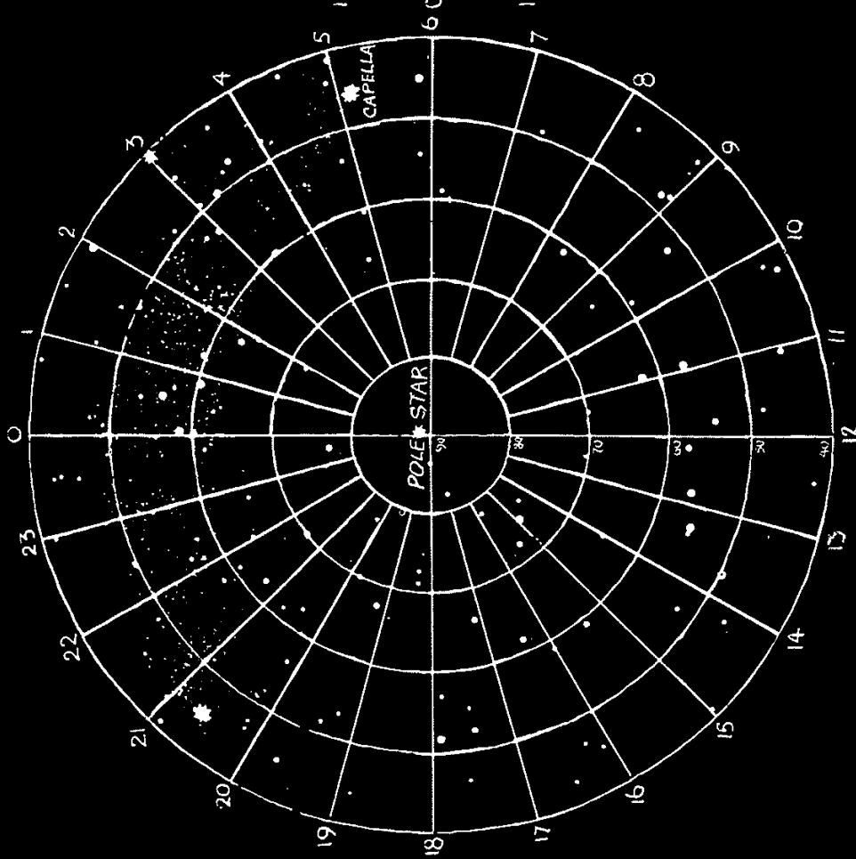
STAR POSITIONS - MIDNIGHT MARCH 2 ND .
