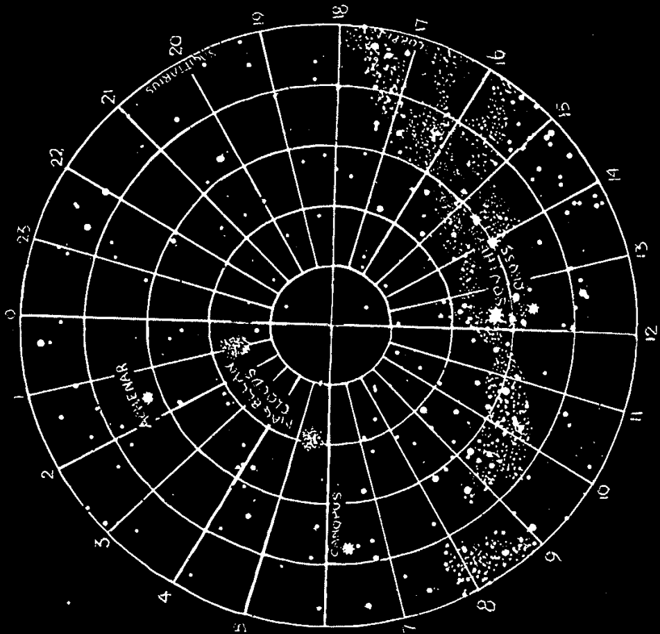
SOUTH POLAR CHART
