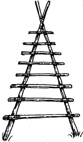
The bush ladder is made in the form of a tepee or extended triangle. At ground level the support poles should be at least 1 metre apart otherwise it will not be stable.
