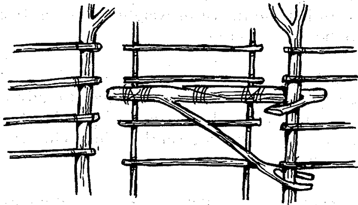
Door frames are 'hinged' by a combination of hook and fork. The method is similar to a campfire swinging frame used to support a billy or other cooking vessel.
