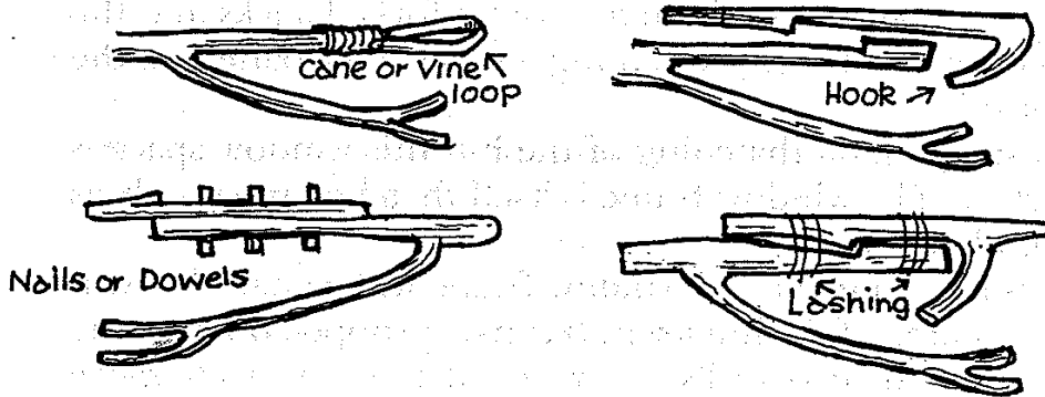
Different methods of assembling the door frame hinge. Top left shows a cane or vine loop used with the forked branch. Top right illustrates how a hook can be cut into a straight branch. The bottom two illustrations show different methods of lashing — the left with nails or dowels and the right by lashing.
