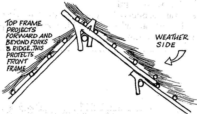
Assembly of thatching on a lean-to shelter. Note how the top frame projects forward and beyond the fork and the ridge itself to protect the front frame.
